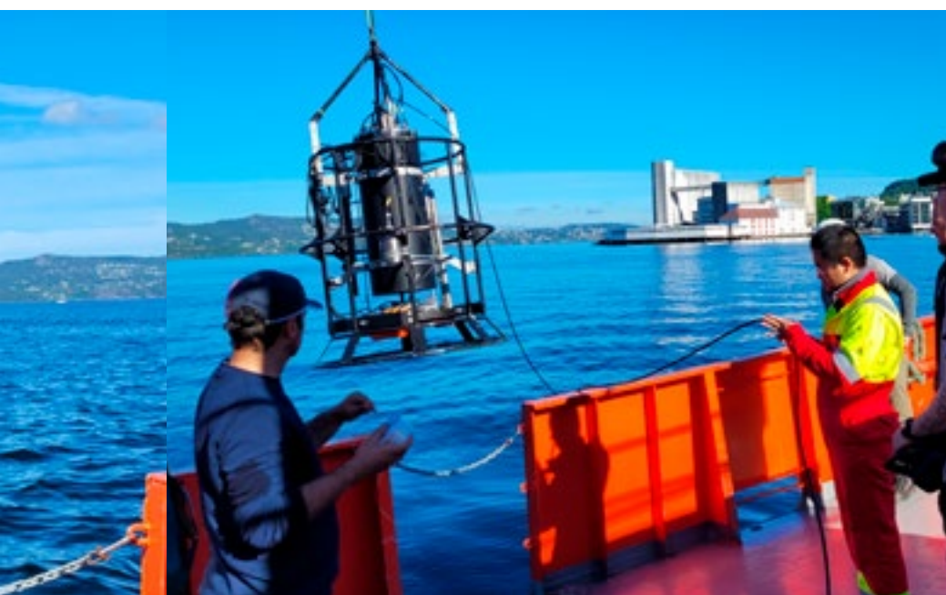
Figure 8. An acoustic probe with 5 echo sounders was used to do experimental measurements on calibration spheres at Sandvikflaket just outside Bergen. Backscatter from two calibration spheres positioned above each other with different separation distance.
